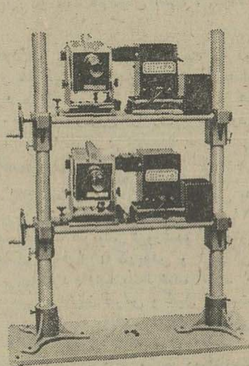
Photo-finish Camera for Athletics and Cycling
