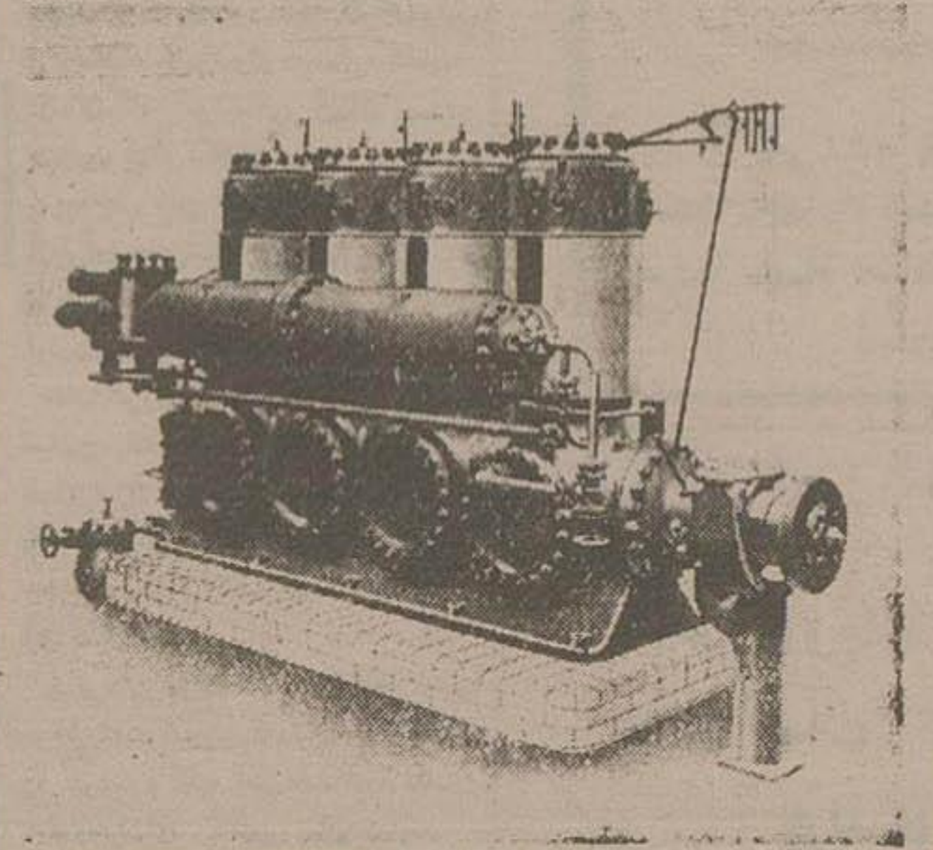
Four-Cylinder mark 4 Z 12 Ammonia compressor
